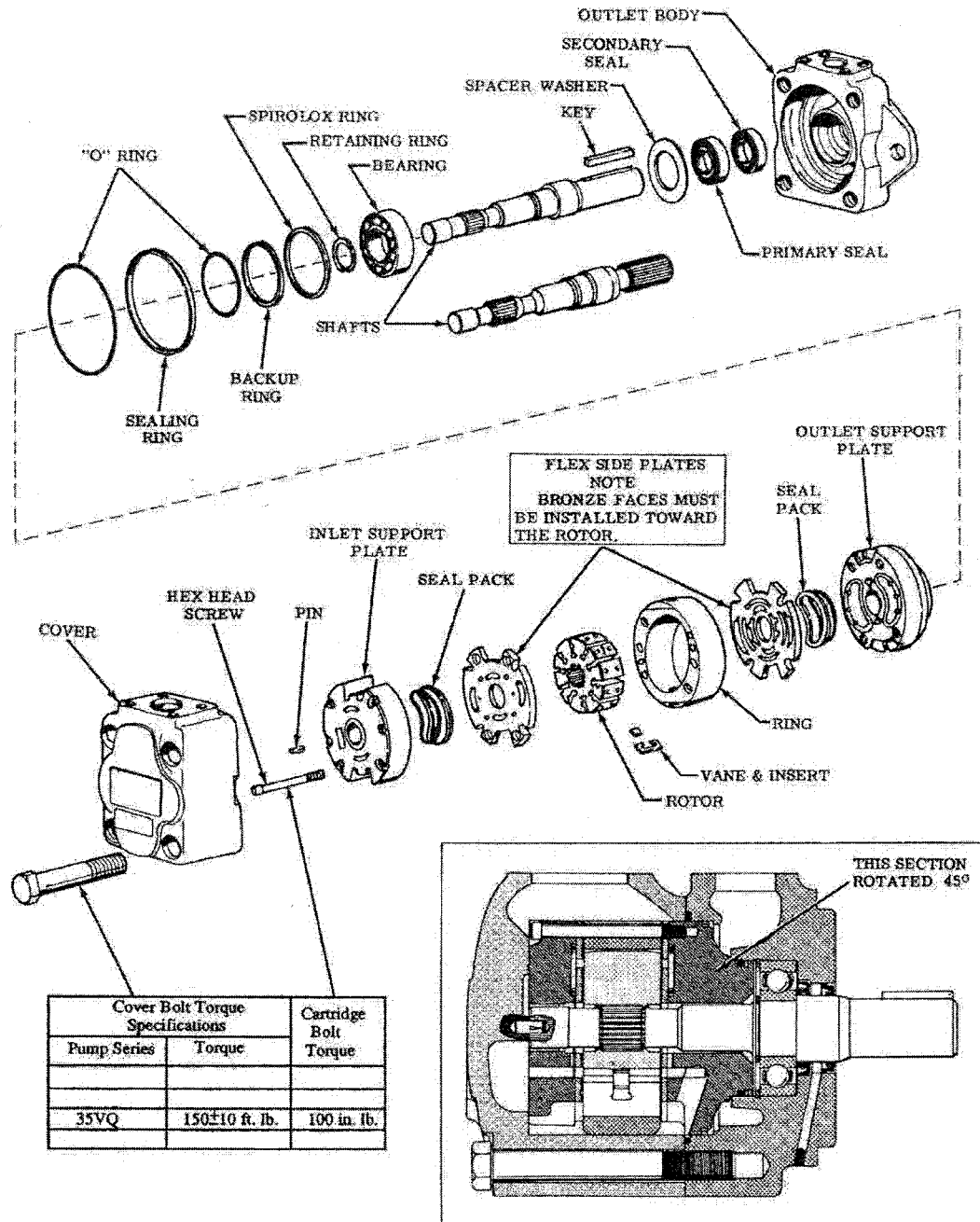
FIG. 2 Pump Components
